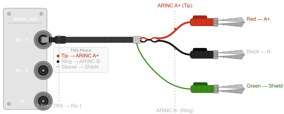
Connection with front box front panel for RX1
