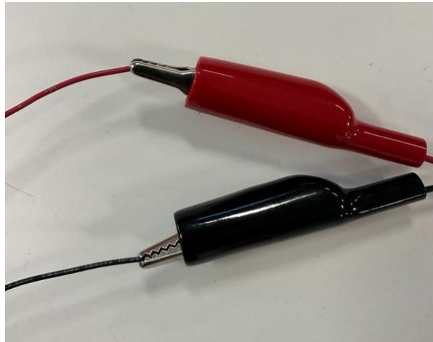
Connection to A+/B- wires of the Aircraft's ARINC 429 BUS
