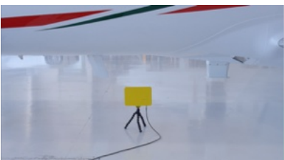
Good line of sight between Aircraft Antenna under test and ARTS 7000 test antenna.
